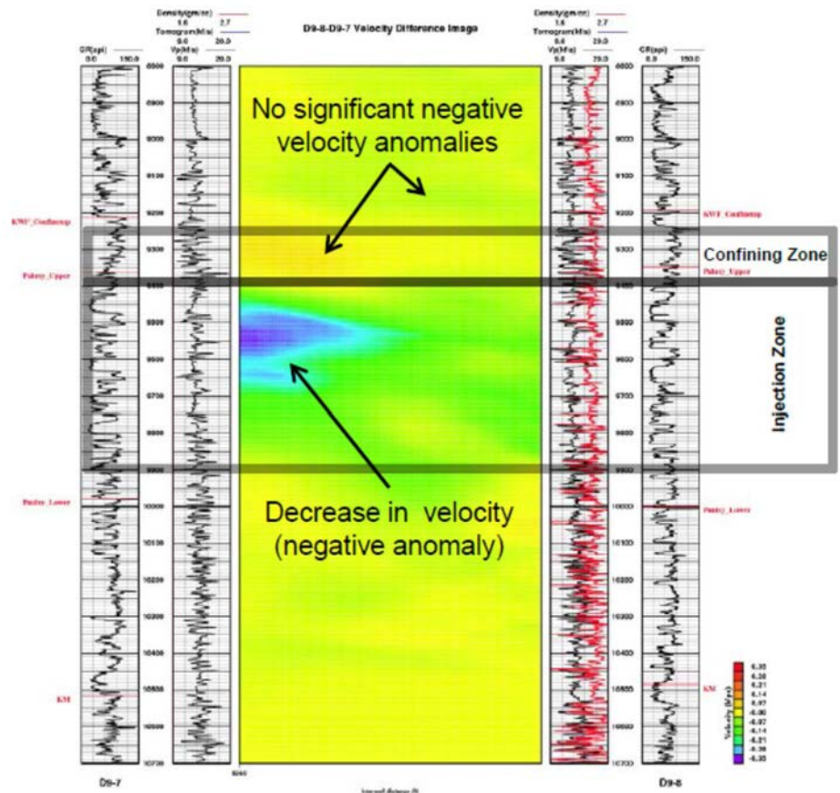
Figure 22. Pixelized difference tomography results without seismic reflection overlay showing positive velocity differences in yellow and negative differences in green and blue
