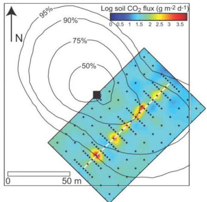
Figure 9: Map of Log Soil CO 2 Flux, Interpolated Based on Measurements Made at the Black Dots on July 25, 2008
