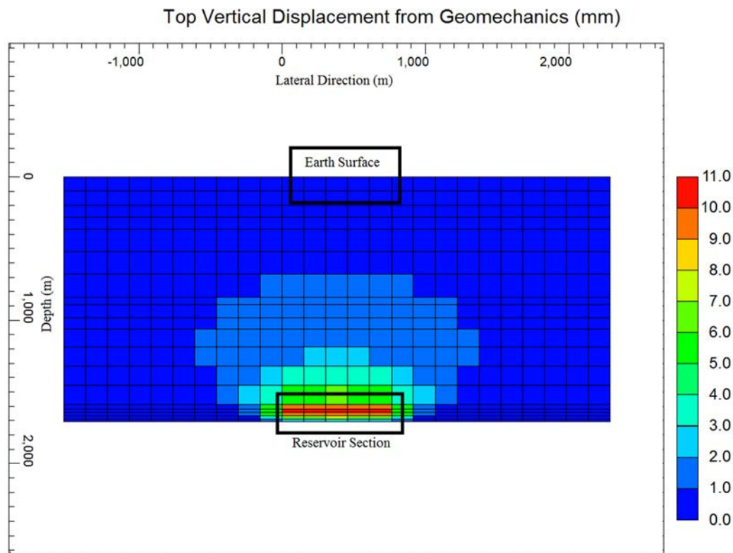
Figure 15: Schematic of Reservoir and Overburden Deformation for Conservative Scenario (Predicts the surface uplift will be less than 1mm when reservoir pressure increases from 780 psi [beginning of MRCSP phase] to 4,000 psi; color-coded scale in mm).
