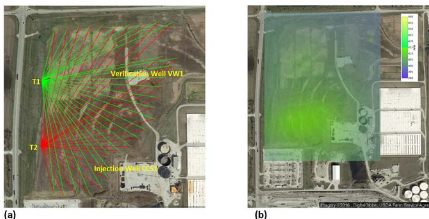
(a) Site layout showing chords from transceivers (T1 and T2) to reflectors. (b) 2-D recreation of the atmospheric CO 2 concentrations collected from the GreenLITE system
