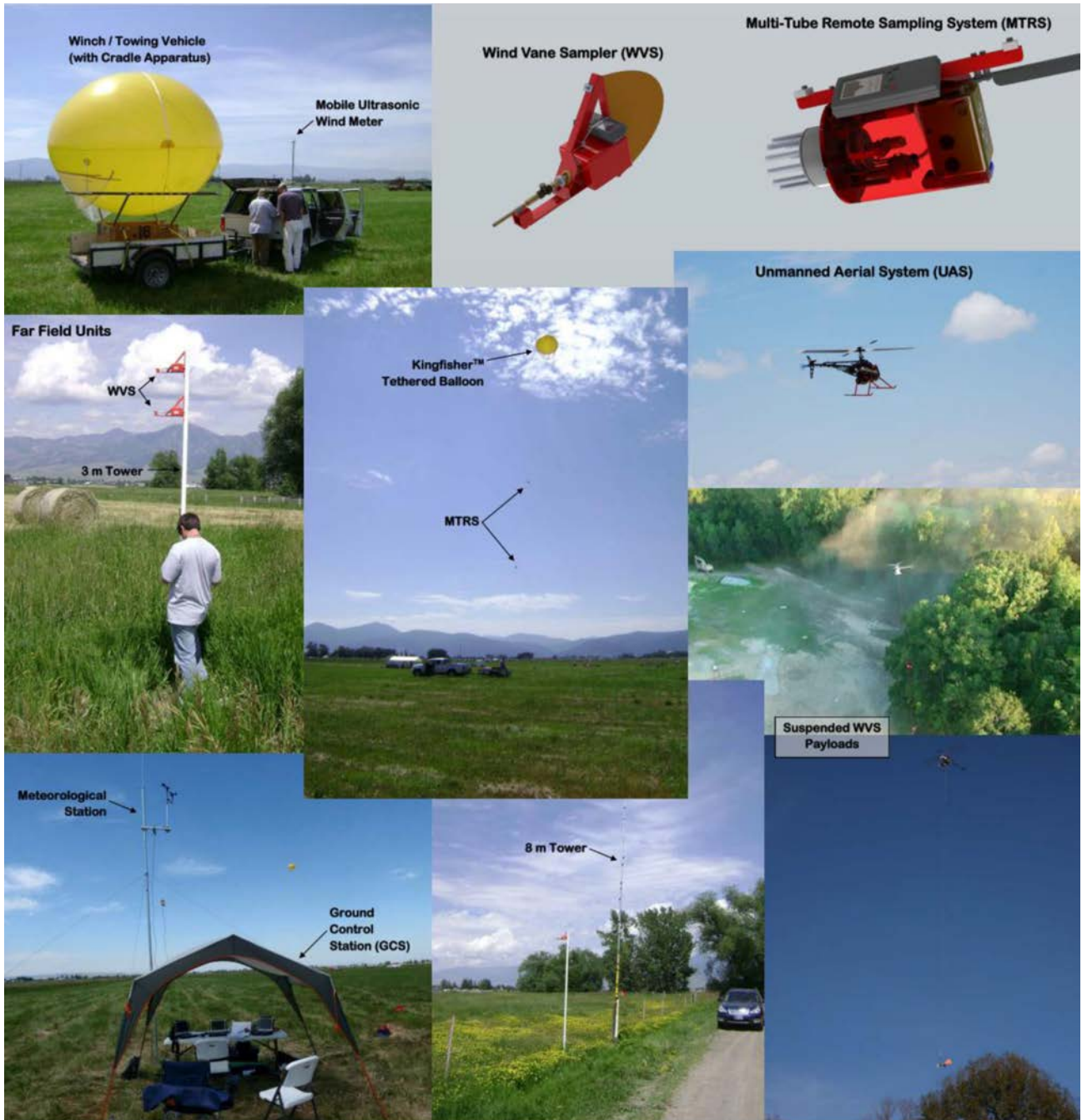
Figure 8: MTRS and WVS Systems for Atmospheric PFT Tracer Monitoring
